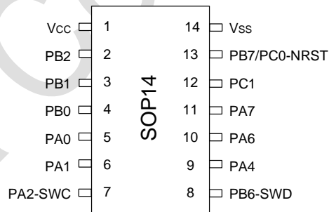
图 3-6 SOP14 Pinout1 PY32F002BD15Sx (Top view)
